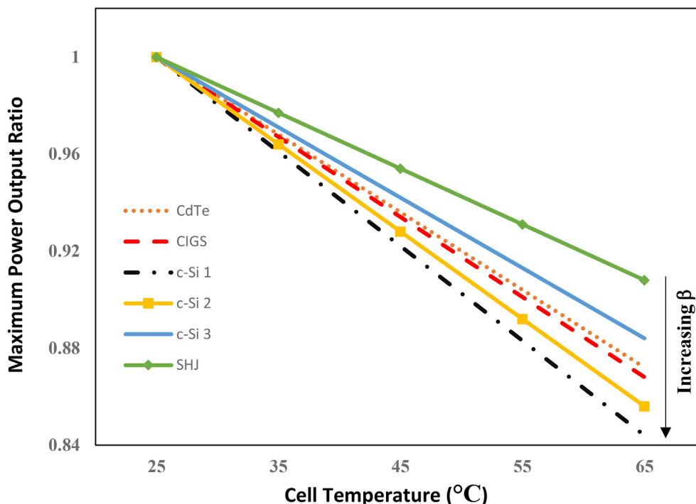
Fig. 5. Photovoltaic module maximum power output ratio (working maximum power relative to maximum power under standard operating conditions) as a function of temperature for several PV module technologies. The values are normalized to standard test conditions (STC) to show the temperature dependence of different PV technologies more clearly.
