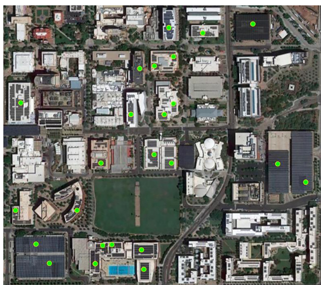
Fig. 1. Photovoltaic systems applied to existing rooftops and parking structures on the campus of Arizona State University, Tempe, Arizona, exemplifying building-applied photovoltaic (BAPV) systems. PV systems are denoted with a green dot. (For interpretation of the references to color in this figure legend, the reader is referred to the web version of this article.)
